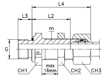
Type: 1049...4 B4 Ring
