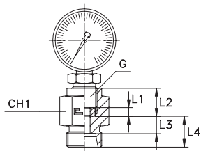
Type: 1059...1 Body Metal washer seal
