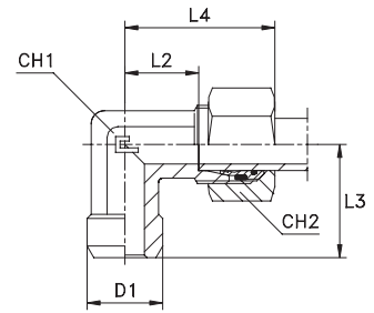
Type: 1058...4 B4 Ring
