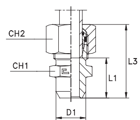
Type: 1055...4 B4 Ring
