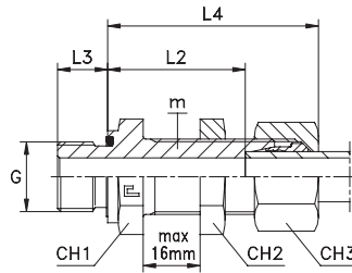
Type: 1049.. B3 Ring
