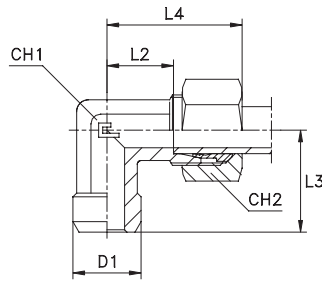
Type: 1058.. B3 Ring
