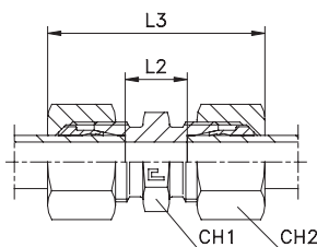
Type: 1035.. B3 Ring
