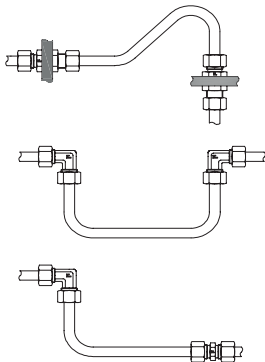
Do not subject the fittings to stress deriving from a poor alignment of the tube which must be able to expand
