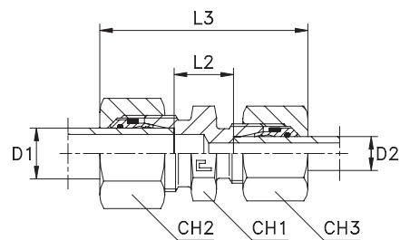
Type: 1041...4 B4 Ring
