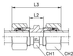
Type: 1035...4 B4 Ring
