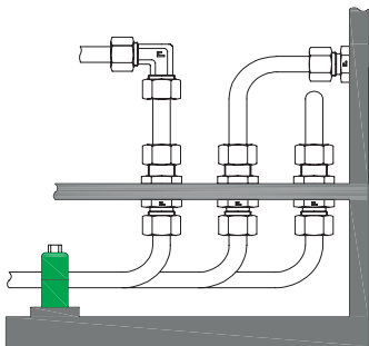
Do not overlay the tubes to facilitate maintenance
