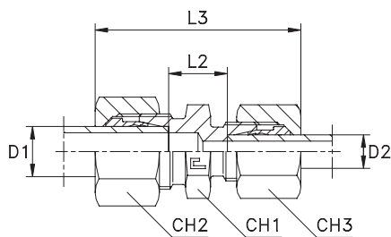
Type: 1041.. B3 Ring
