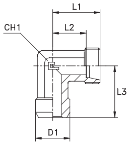
Type: 1058...1 Body
