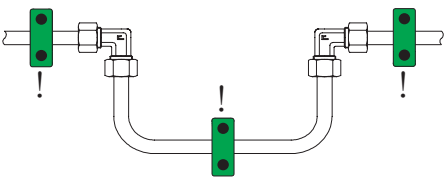
Do not excessively fasten the tubes as these must always be allowed to dilate without any problem
