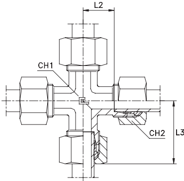
Type: 1040.. B3 Ring
