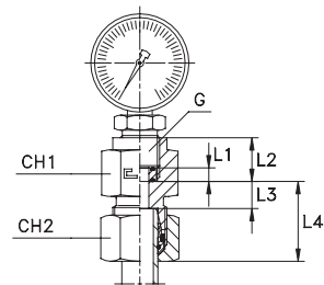
Type: 1059...4 B4 Ring O-ring washer seal
