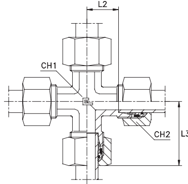
Type: 1040...4 B4 Ring
