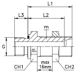
Type: 1049...1 Body
