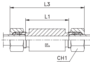
Type: 1056.. B3 Ring
