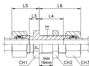
Type: 1036...4 B4 Ring
