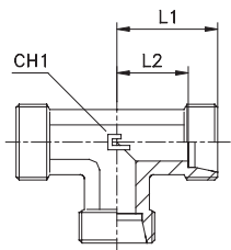
Type: 1039...1 Body
