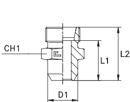
Type: 1055...1 Body
