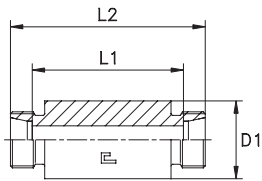
Type: 1056...1 Body
