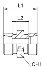
Type: 1035...1 Body
