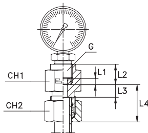
Type: 1059.. B3 Ring Metal washer seal
