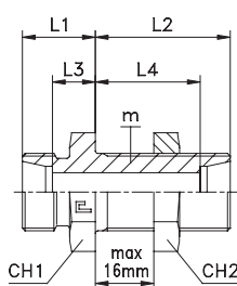
Type: 1036...1 Body
