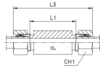
Type: 1056...4 B4 Ring
